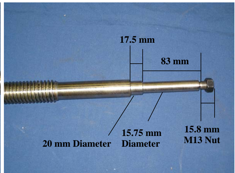
Right hand side screw with 1 bearing
